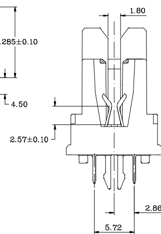
Section X-X
