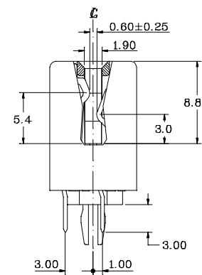
Section X-X
