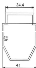
45° CABLE ENTRY
