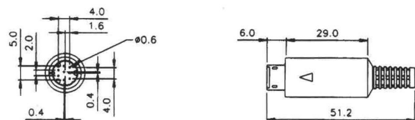
MOLDED TYPE (MALE)
