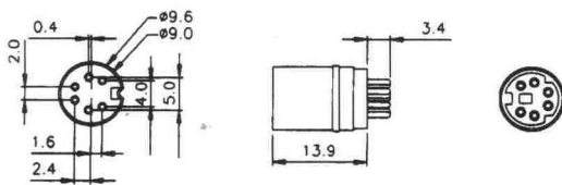
MOLDED TYPE (FEMALE)
