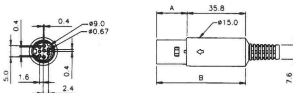
ASSEMBLY TYPE (FEMALE)
