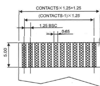
FPC/FFC t = 0.30 \pm 0.05
