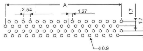
P.C. BOARD LAYOUT PATTERN
