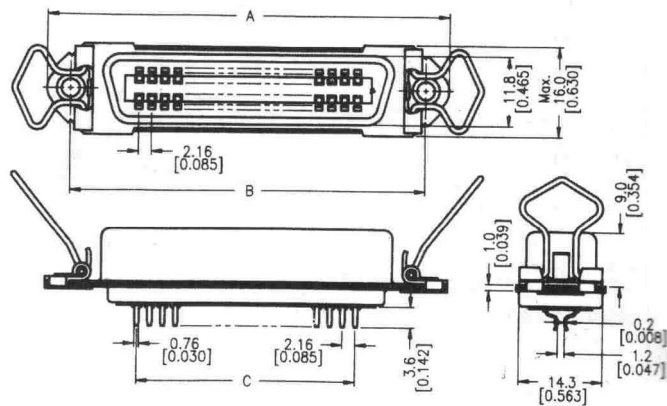
57S(P)-40 Series (Female)
