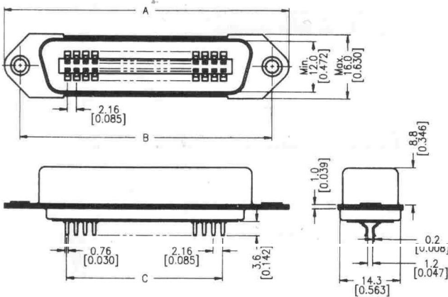
57S(P)-20 Series (Female)
