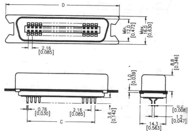
57S(P)-40 Series (Female)
