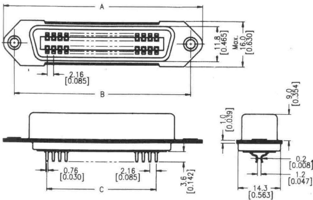
57S(P)-20 Series (Female)
