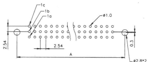
R TYPE (MALE-STRAIGHT)
