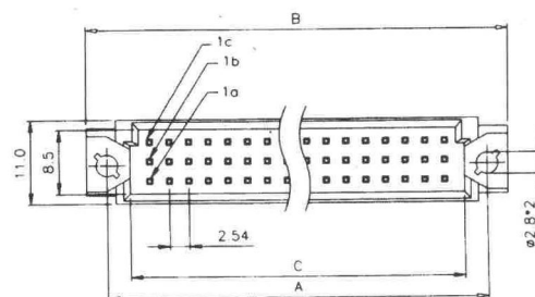
C TYPE (MALE-RIGHT ANGLE)
