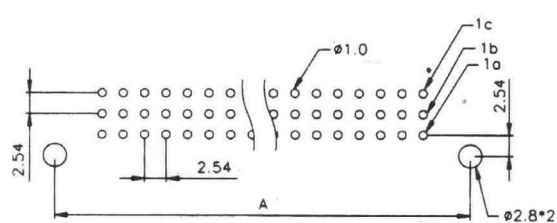
R TYPE (FEMALE-RIGHT ANGLE)
