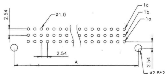
C TYPE (MALE-RIGHT ANGLE)
