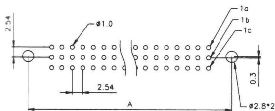
C TYPE (FEMALE-STRAIGHT)
