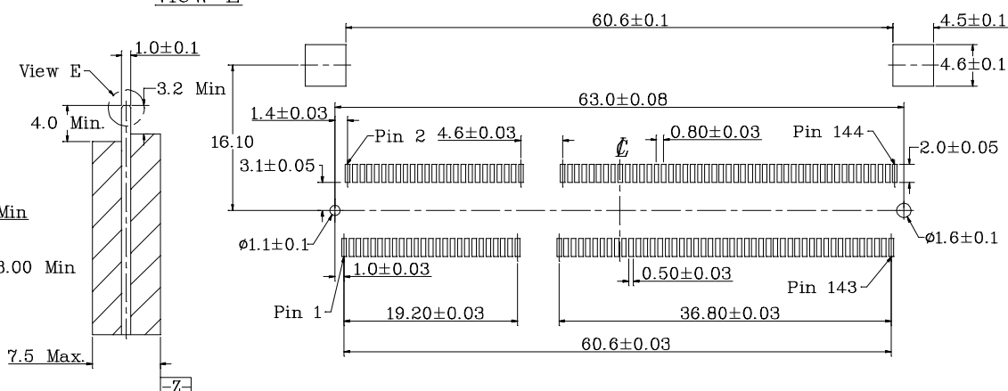
Recommended P.C.B. PAD Layout
