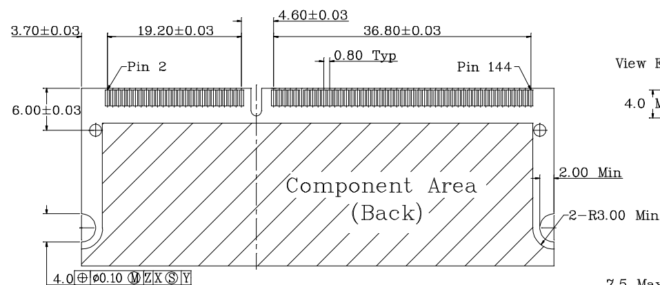
Circuit Position Of S.O.DIMM
