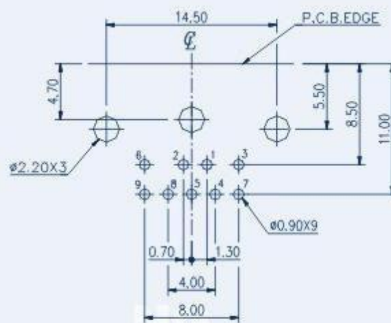
P.C.B. RECOMMEND LAYOUT (BOTTOM VIEW)
