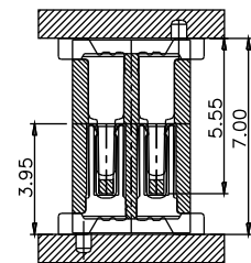
2065P-XXG-550 and 2065S-XXG-390 Mating Height 7.0mm
