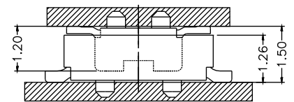
2004P-XXG-120 and 2004S-XXG-126 Mating Height 1.5mm
