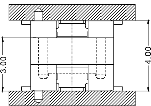
2000P-XXG-330-018 and 2001S-XXG-300-018 Mating Height Draw(Ref)
