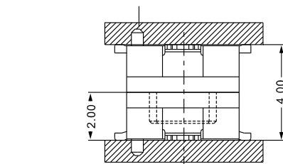
2000P-XXG-330-017 and 2001S-XXG-200-017 Mating Height Draw(Ref)
