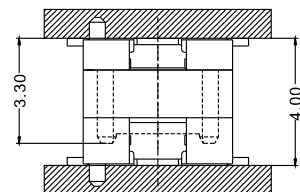
2000P-XXG-330-018 and 2001S-XXG-300-018 Mating Height Draw(Ref)
