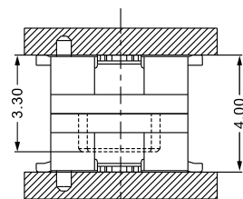
2000P-XXG-330-017 and 2001S-XXG-200-017 Mating Height Draw(Ref)
