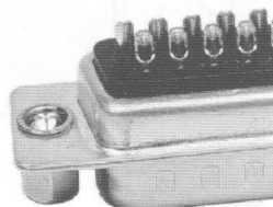
D 前壳上铆接螺母带UNC4-40(盲孔) Screw riveted to front shell with UNC4-40 (blind-hole)
