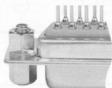
B 后铆接螺母带反双头螺丝UNC4-40 Nut riveted rear shell with anti-dualhead screw UNC4-40
