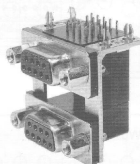
2 UNC4-40锁紧螺丝(双层) Screw lock UNC4-40(Dual Port)
