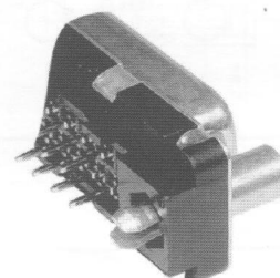
E 前螺母UNC4-40后鱼叉 Front nut/rear harpoon UNC4-40
