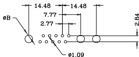
PCB LAYOUT
