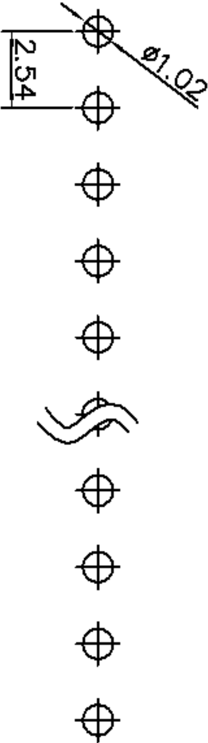
PCB Layout
