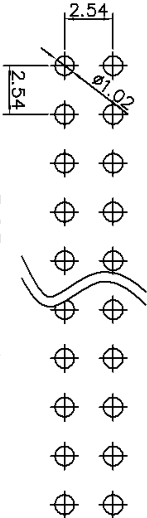
PCB Layout
