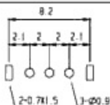
PCB LAYOUT
