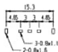
PCB LAYOUT
