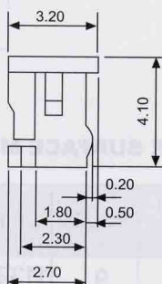
B-B SECTION
