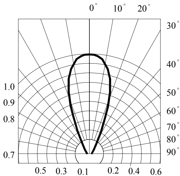
RADIATION DIAGRAM
