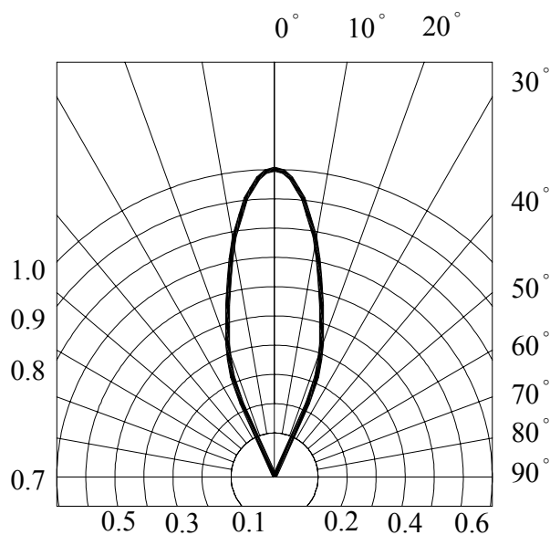
RADIATION DIAGRAM
