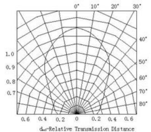
Figure 6. Directivity
