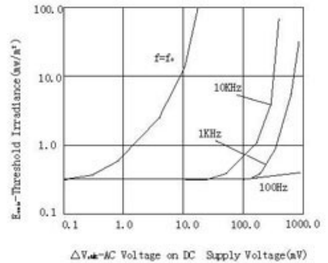
Figure 2. Sensitivity vs. Supply Voltage Disturbances
