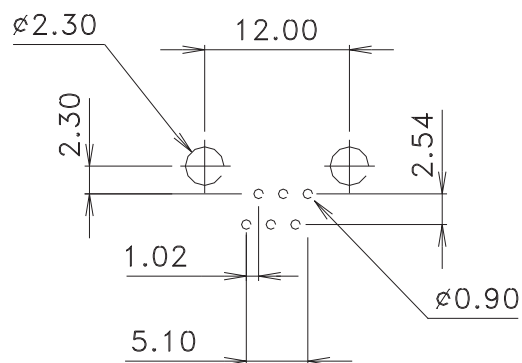
PCB LAYOUT
